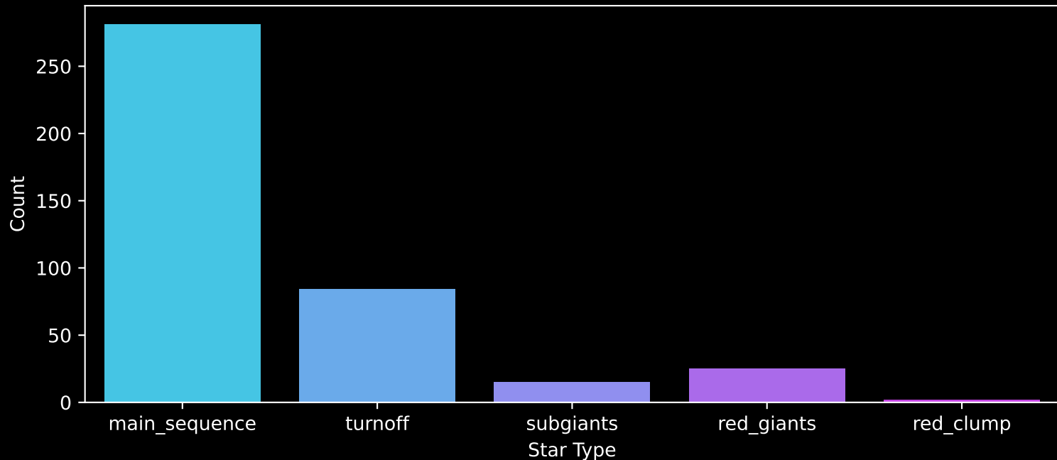
GALAH DR4 Field: [6689] Count plot of Star Type
