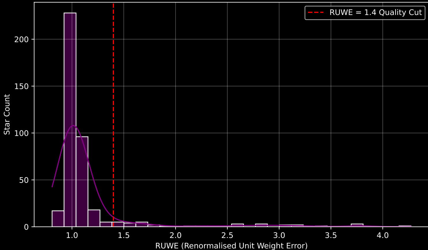
GALAH DR4 Field [6689] RUWE Distribution (n= 399)
