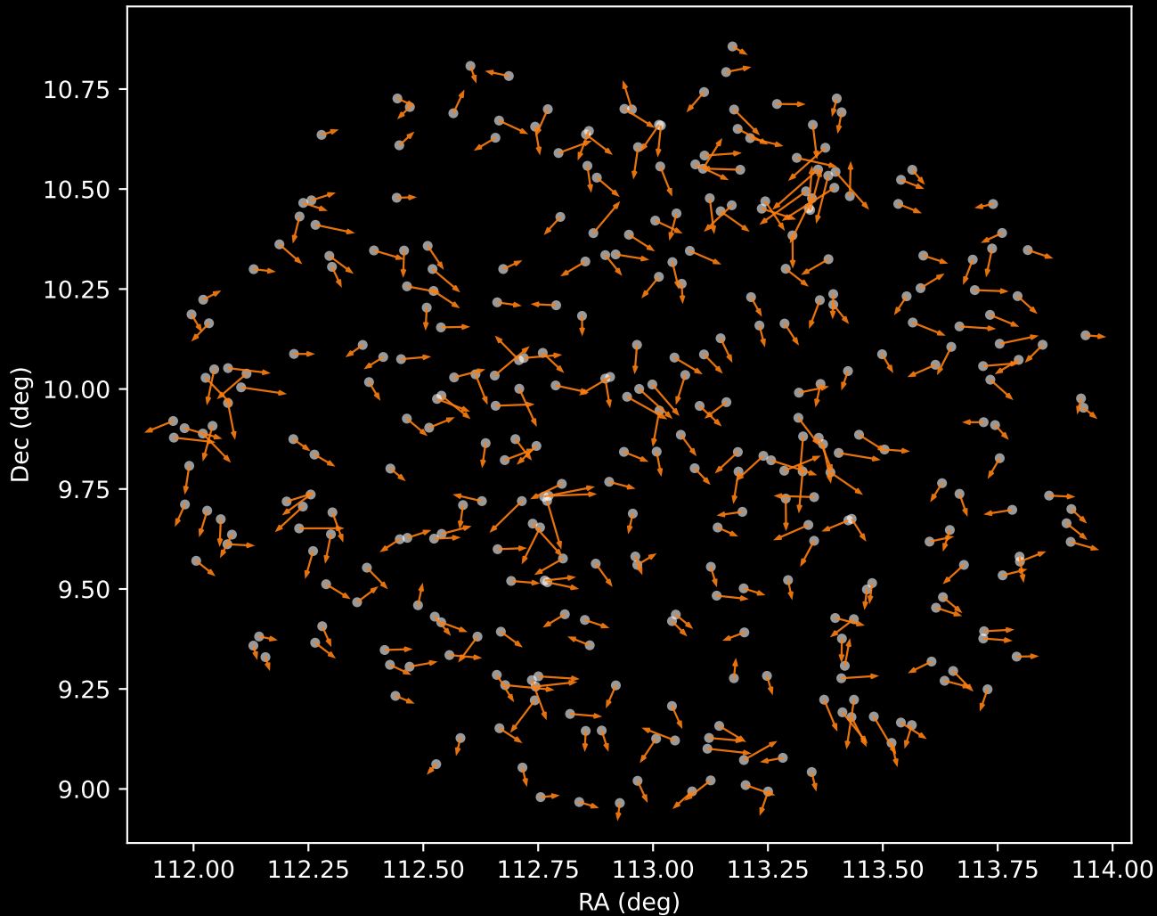
GALAH DR4 Cluster 2 Proper Motion Vectors (n=340)
