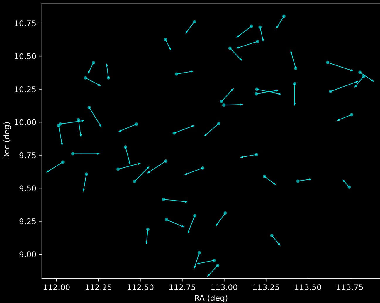
GALAH DR4 Noise Stream Proper Motion Vectors (n=50)
