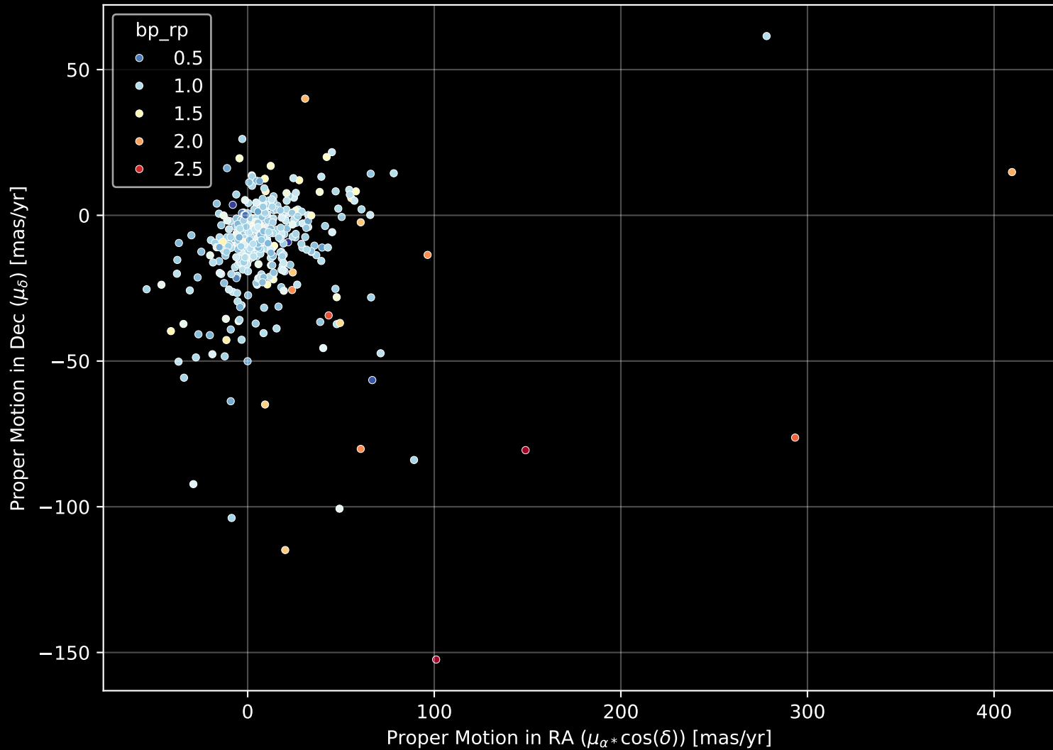
GALAH DR4 Field: [6689] Proper Motion Diagram (n= 407)
