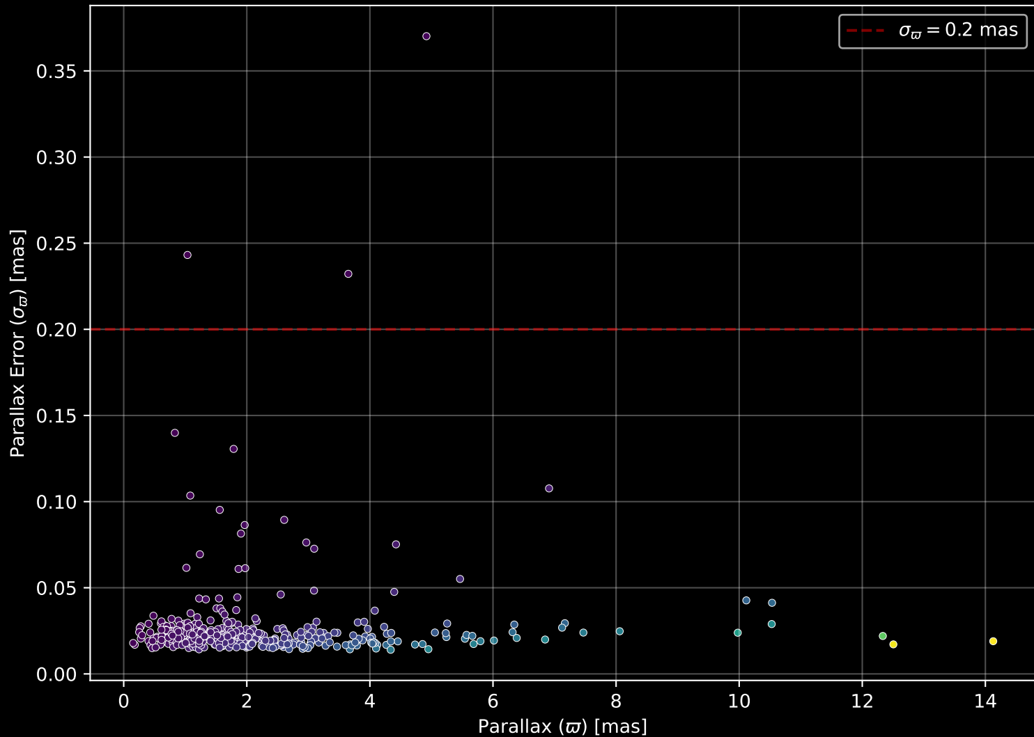
GALAH DR4 Field: [6689] Parallax Quality (n= 407)
